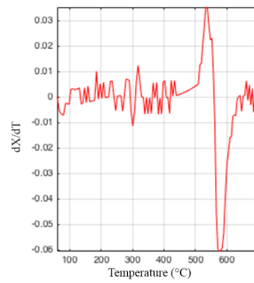
CH160106 First Derivative (heating & cooling)
