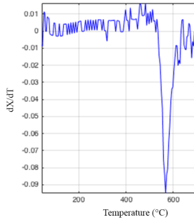
CH160110 First Derivative (heating & cooling)
