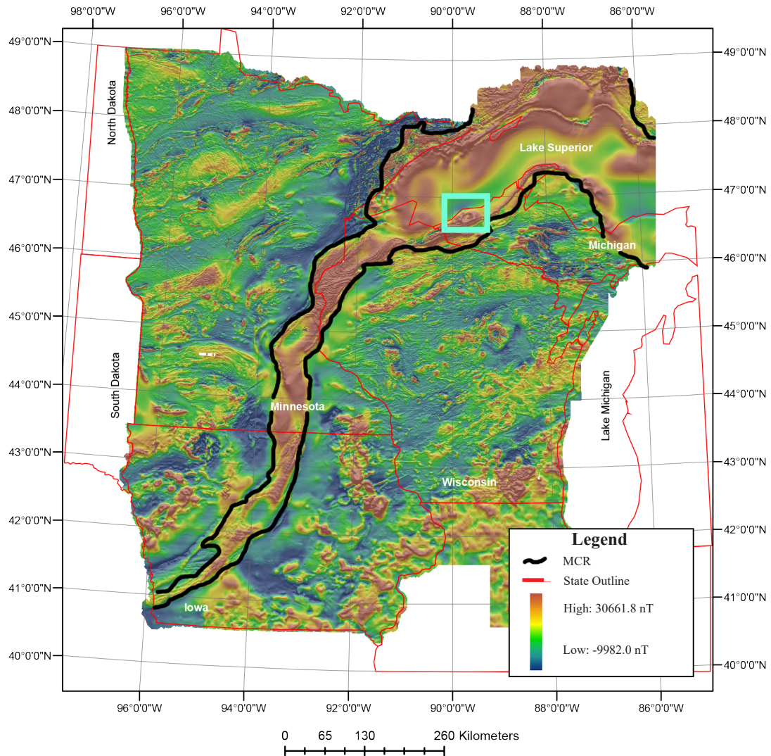
Figure 3: Aeromagnetic survey of the MCR
