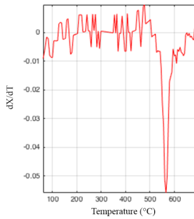
CH160202 First Derivative (heating & cooling)
