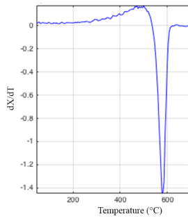
CH160108 First Derivative (heating & cooling)
