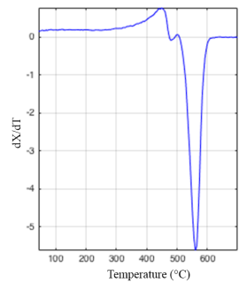
CH160102 First Derivative (heating & cooling)
