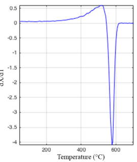
CH160105 First Derivative (heating & cooling)
