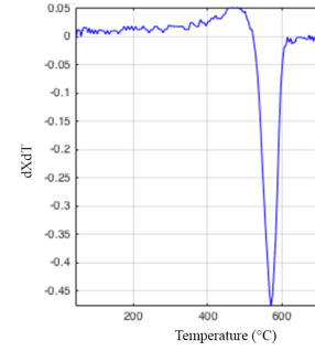
CH160201 First Derivative (heating & cooling)
