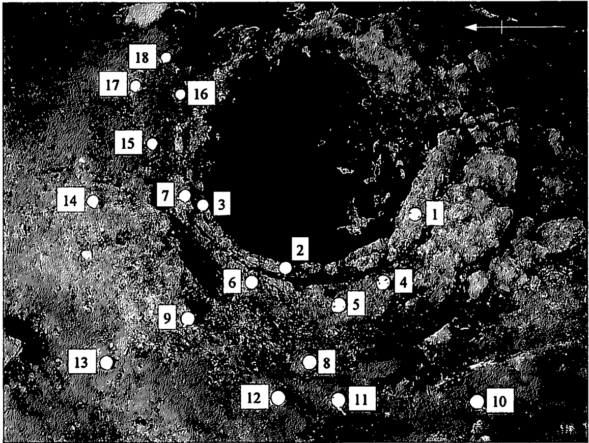
Figure 2. Hagg End, Bilsdale, N. Yorks.: Trench 1 iron smelting furnace (contexts 135 to 141) archaeomagnetic dating sampling points.
