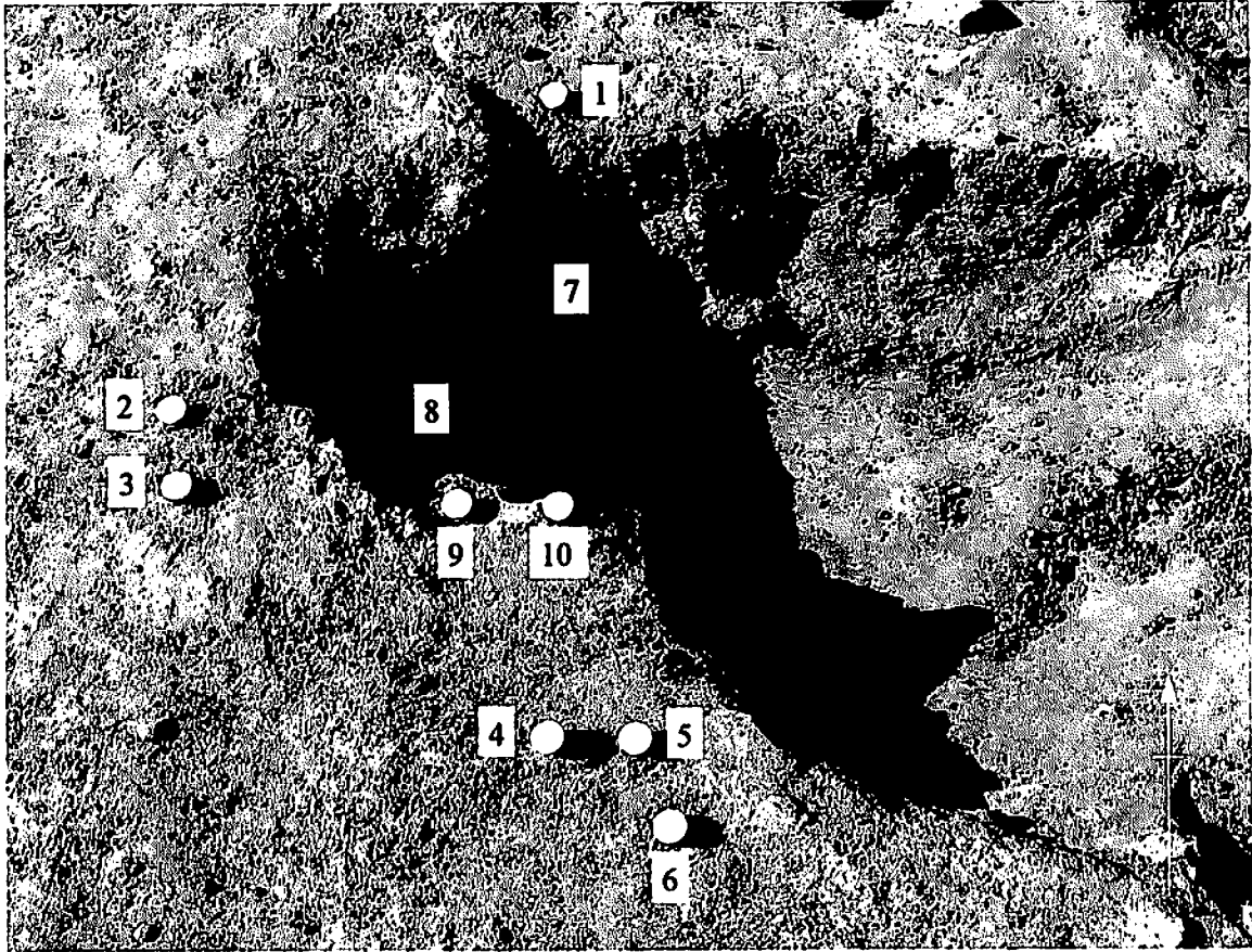
Figure 4. Ewecote, Bilsdale, N. Yorks.: Trench 1 furnace feature archaeomagnetic dating sampling points.
