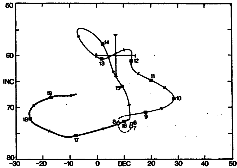
Figure 6: Corrected mean remanence vectors for the Hagg End HE03 Trench 1 iron smelting furnace together with 95% confidence level errors, superimposed on the British archaeomagnetic calibration curve (Clark et al. , 1988), normalised to Meriden, showing (upper) 1000BC-AD600 and (lower) AD600-AD1975.
