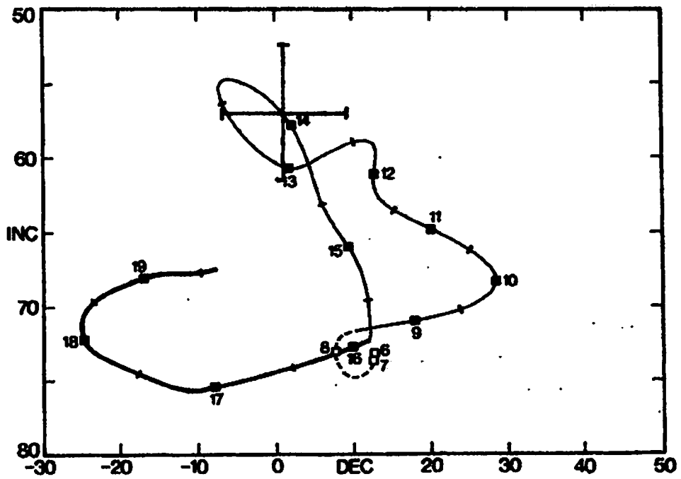
Figure 8: Corrected mean remanence vectors for the Ewecote EC03 Trench 2 iron smelting furnace together with 95% confidence level errors, superimposed on the British archaeomagnetic calibration curve (Clark et al. , 1988), normalised to Meriden, showing (upper) 1000BC-AD600 and (lower) AD600-AD1975.
